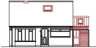
PROPOSED SOUTH-WEST ELEVATION (1:100)
