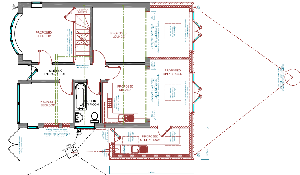
PROPOSED GROUND FLOOR LAYOUT PLAN (1:50)
