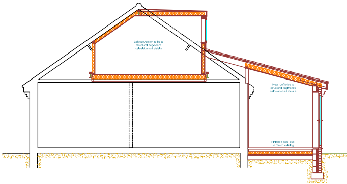
PROPOSED TYPICAL SECTION (1:50)
