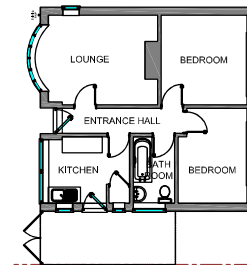
EXISTING LAYOUT PLAN (1:100)
